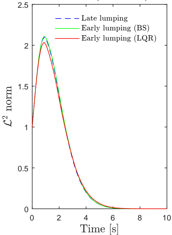
\mathcal{L}^2 -norm (10 modes)
