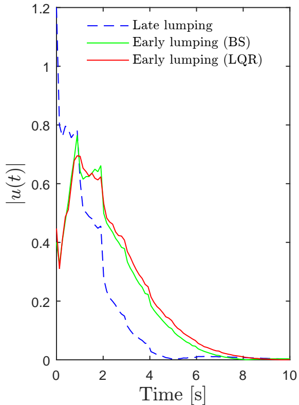
Control effort
