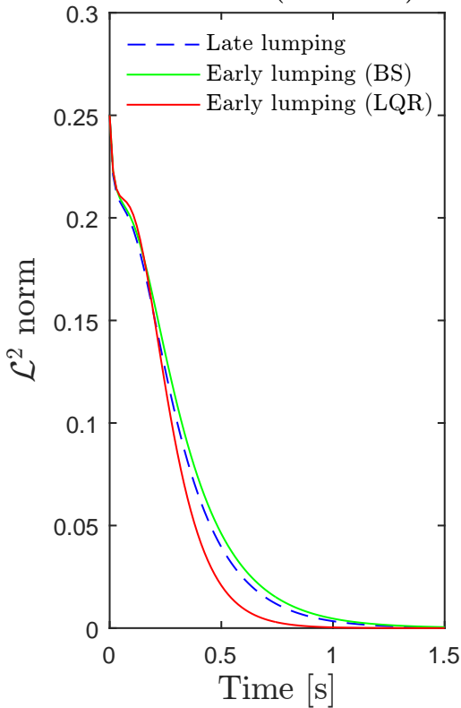
\mathcal{L}^2 -norm (5 modes)
