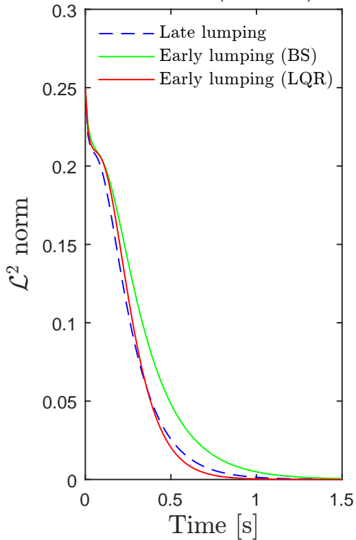
\mathcal{L}^2 -norm (1 mode)
