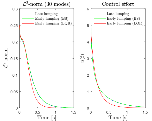
Fig. 3. Time evolution of the \mathcal{L}^2 -norm and of the control efforts for different controllers (heat equation, N=30 , M=30 )
