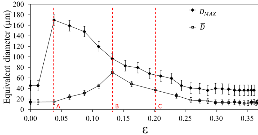
Figure 4: Evolution of the maximum and average grain sizes along the strain gradient of a sample deformed at 1040^{\circ}\text{C} , \dot{\varepsilon} = 0.01 \text{ s}^{-1} and solution-treated for one hour. Landmark \varepsilon^A : first overgrown grain; Landmark \varepsilon^B : microstructure fully replaced by overgrown grains; Landmark \varepsilon^C : fine and homogeneous microstructure.
