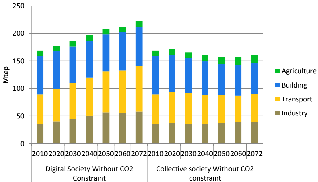
Figure 1: Final energy consumption for "Digital Society" and "Collective Society" lifestyle scenarios
