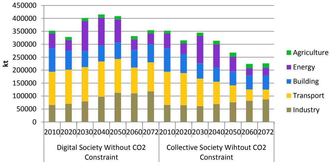
Figure 2 : CO 2 emissions for "Digital Society" and "Collective Society" lifestyle scenarios
