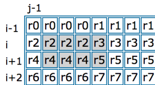
Figure 12: Data layout illustration for double-row computation
