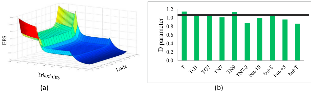
Fig. 4. (a) representation of the fitted failure surface (in the space of Lode parameter, triaxiality, and strain to fracture) of the new exponential failure criterion; (b) prediction of damage for the 10 experimental tests.
