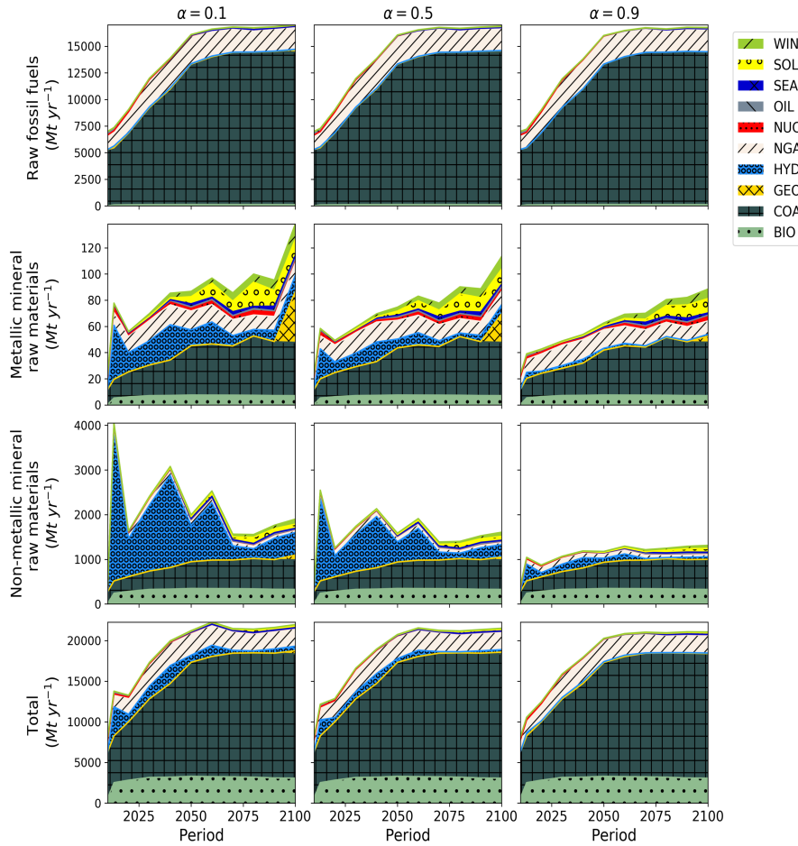
Figure 6. Total annual mass of fossil fuels, metallic and non-metallic raw mineral materials used by power generating technologies at \alpha = 0.1 , \alpha = 0.5 , and \alpha = 0.9
