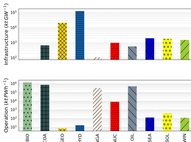
Figure 4. Materials requirements in the infrastructure (construction + dismantling) and operation phases of main electricity generation technologies (BIO: biomass, COA: coal, GEO: geothermal, HYD: hydro; OIL: oil, NGA: natural gas, NUC: nuclear, SEA: marine, SOL: solar, WIN: wind). The values are averaged on regions and periods
