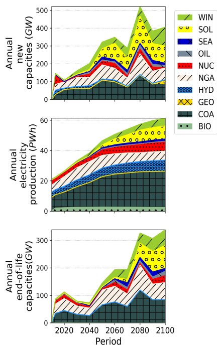
Figure 3. Annual new capacities (NCAP), electricity production (PROD) and end-of-life capacities (RCAP). The global electricity mix is represented by 10 technology categories (BIO: biomass, COA: coal, GEO: geothermal, HYD: hydro; OIL: oil, NGA: natural gas, NUC: nuclear, SEA: marine, SOL: solar, WIN: wind)
