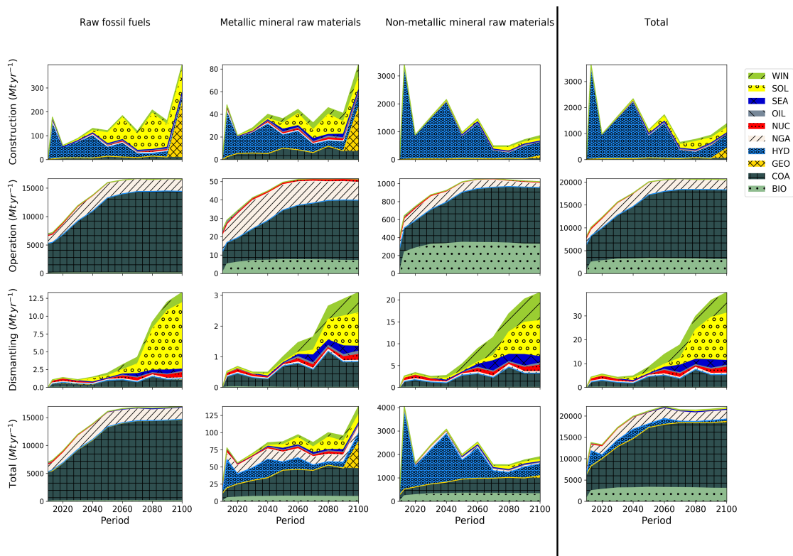
Figure 5. Total annual mass of fossil fuels, metallic, and non-metallic mineral raw materials needed in the construction, operation, and dismantling phases, \alpha = 0.1
