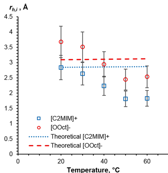
Figure 5. Stokes-Einstein radii of the cation and anion in [\text{C}_2\text{MIM}][\text{OOct}] as a function of temperature (points), as follows from Fig. 4b and Eq. 4. Dashed lines correspond to cation and anion sizes calculated from Eq. 1.
