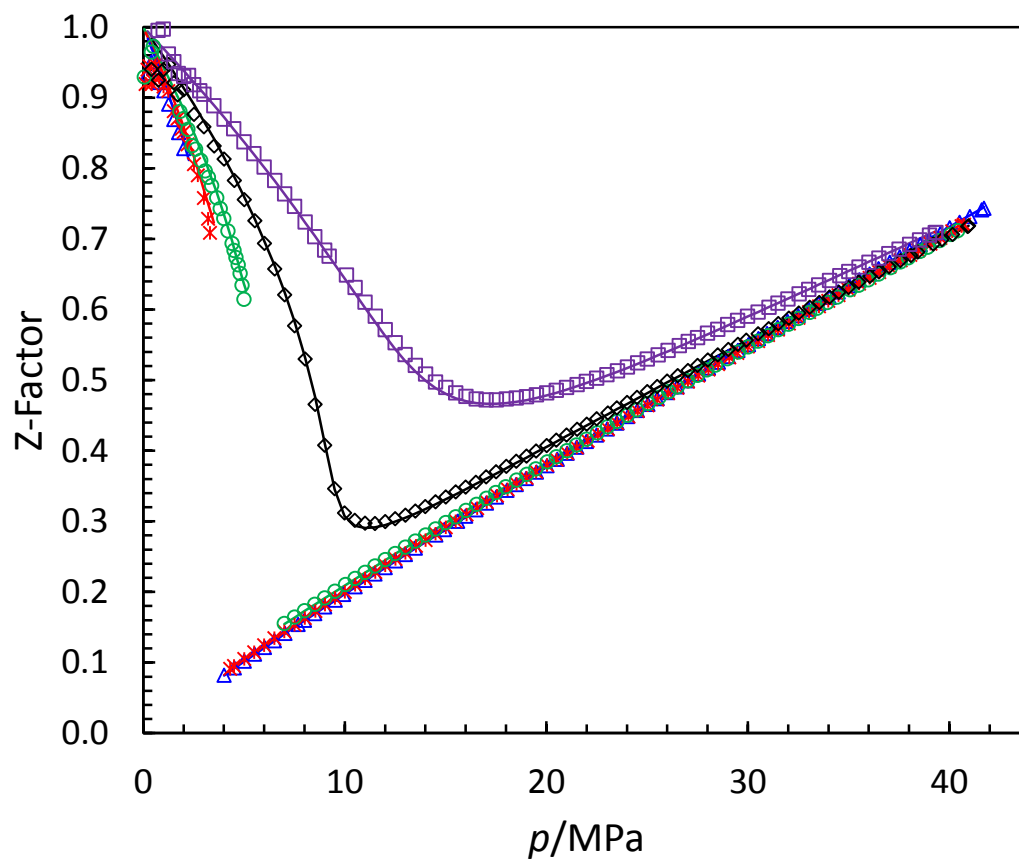
Figure 5 – Compressibility factor of the CO 2 – SO 2 system. Experimental results: (Δ) 273. 15 K, (*) 283.15 K, (◇) 323.15 K and (□) 353.15 K for the 0.9503 mole CO 2 + 0.0497 mole SO 2 and (○) 298.15 K for the 0.9478 mole CO 2 + 0.0522 mole SO 2 . Lines: Predictions using the multi parameter EoS
