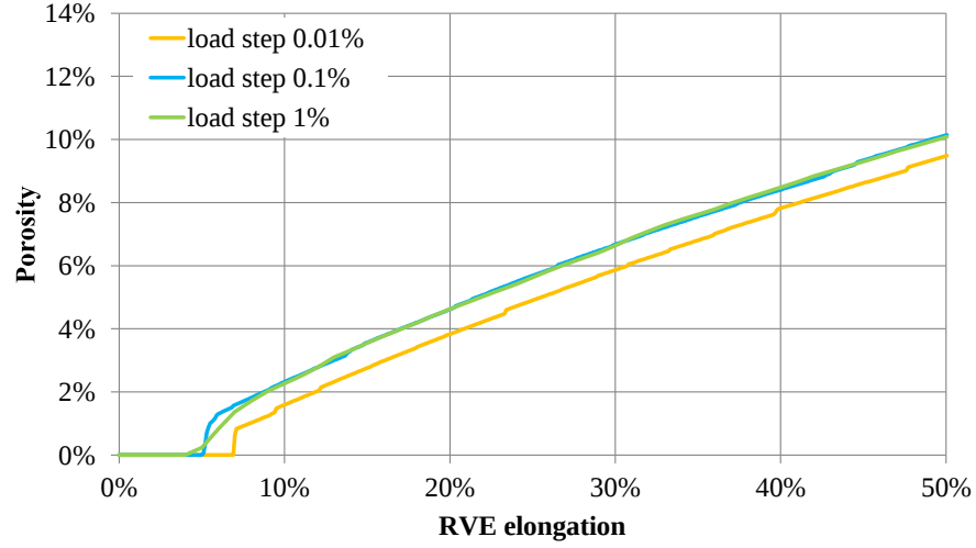
Figure 20: Sensitivity of the porosity during loading with respect to the load step.
