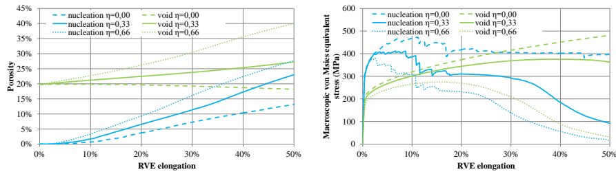
(a) Porosity change for the three simulations. (b) Macroscopic von Mises equivalent stress change for the three simulations.
