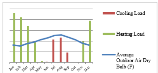
Figure 8. Heating and cooling monthly load profiles
