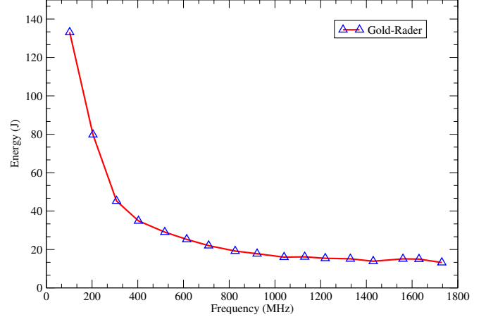
Fig. 2. Energy vs. Frequency: energy consumption for the Gold-Rader bit-reverse algorithm with varying clock frequency on an Nvidia Jetson TX1.
