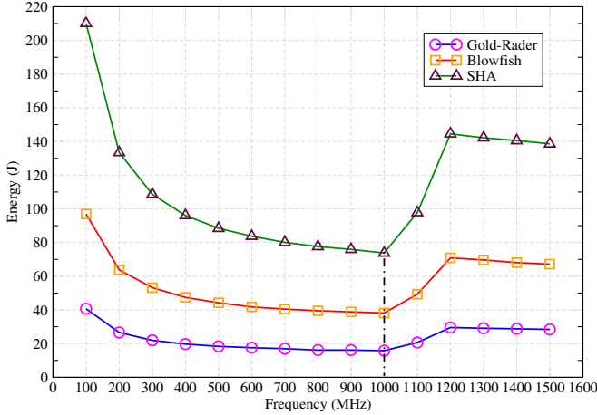
Fig. 8. Total energy vs. Frequency: energy consumption of our three benchmarks with varying clock frequency on the TI AM572x platform. The dotted line represents the optimum frequency for each of the benchmarks.
