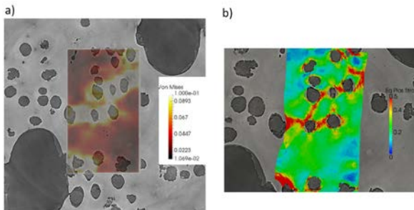
Figure 1 comparison of the equivalent strain field for a) an incremental DVC correlation and b) the total strain field for a micromechanical simulation using measured boundary conditions
