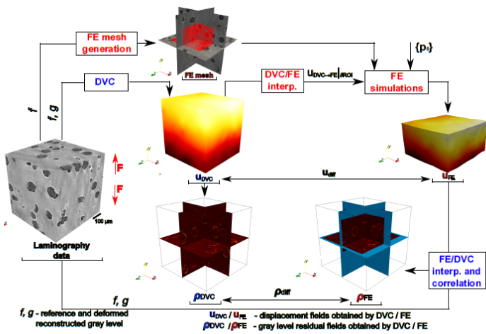
Figure 1 framework for micromechanical simulations based on synchrotron 3D imaging and comparison with volume field measurements (DVC) [Buljac 2017]
