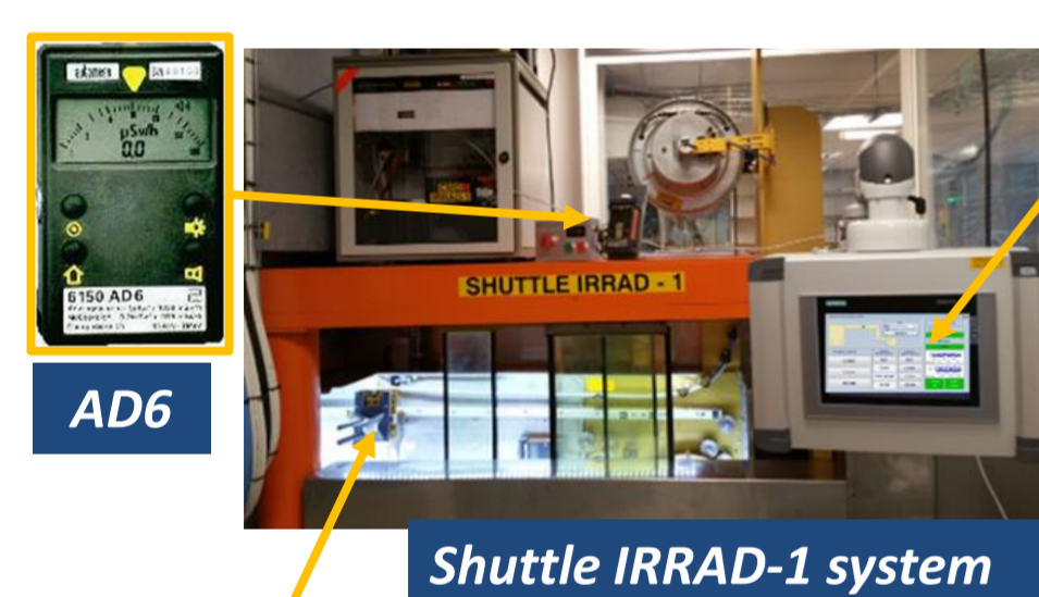
Shuttle IRRAD-1 system
