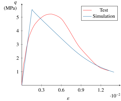
Figure 5. Comparison of strain-stress curves for uniaxial compression test
