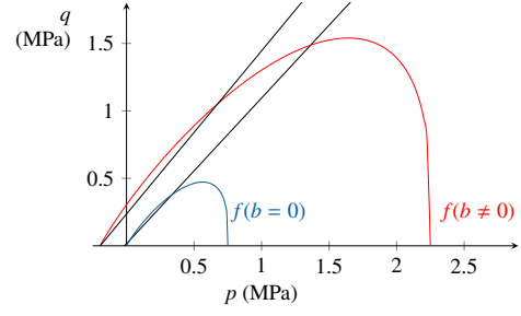
Figure 2. Yield surfaces in the (p, q) plane
