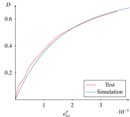
Figure 6. Evaluation of the damage law
