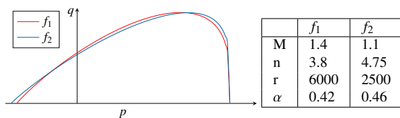
Figure 4. Redundancy forecast in the parameters space
