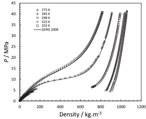
Fig. 6. Experimental and modelling results of CO 2 - H 2 S at different isotherms, experimental results: ( \Delta ) 273.15 K, ( * ) 283.15 K, ( \circ ) 298.15 K, ( \diamond ) 323.15 K and ( \square ) 353.15 K. Lines: Predictions using the GERG-2008 EoS
