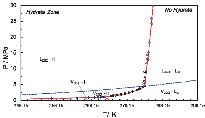
Fig. 4. Example of CO 2 phase diagram with the hydrate zone from Chapoy et al. [6].
