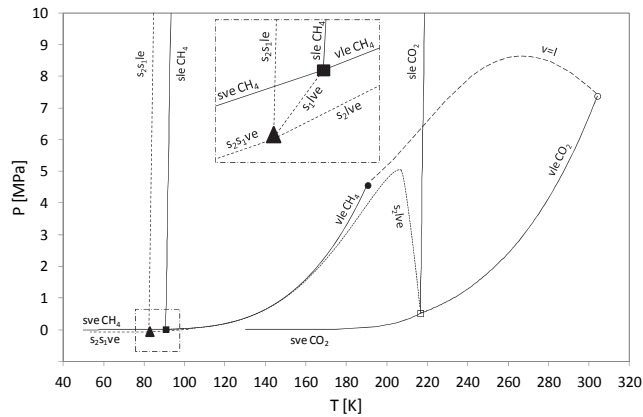
Fig. 3. CH 4 – CO 2 phase diagram (from [5]).
