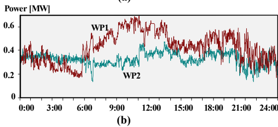
Figure 3 : Operation of the Lemnos power system on Feb. 10, 1994.
