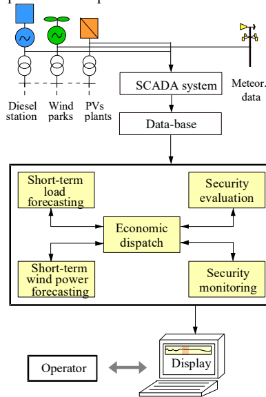
Figure 1 : The control system architecture.
