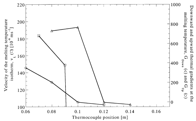
Fig. 5. Average velocities of the melting temperature isotherm, v_L , calculated between two thermocouples (left scale) and thermal gradients ahead, G_{Up} , and below, G_{Down} , the position of the thermocouples at the time they are reached by the melting temperature (right scale), using the experimental and simulated cooling curves recorded in the 99.99 wt% Al ingot (Fig. 3).
