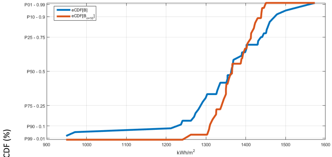
Figure 5.2. Examples of empirical CDFs estimated from the historical data set of yearly direct normal irradiations \{B(y_k)\}_{k \in [1,nd]} (in blue) and the historical data set of 10-years average direct normal irradiations \{B_{n=10}(y_k)\}_{k \in [n+1,nd]} .
