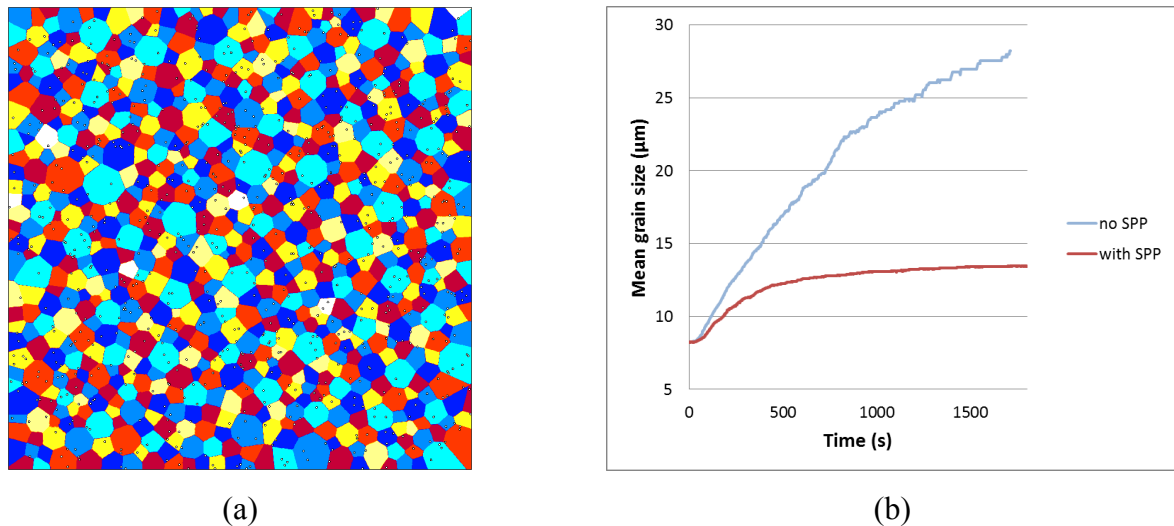
Figure 6. (a) 2D RVE composed of 800 grains (mean grain size of 8\mu\text{m} ) and 1% surface fraction SPP (mean particles radius of 400\text{nm} ); (b) grain size evolution with and without SPP considering an Inconel® 718 alloy held at 985^\circ\text{C} during 30min calculated by the DIGIMU® software.
