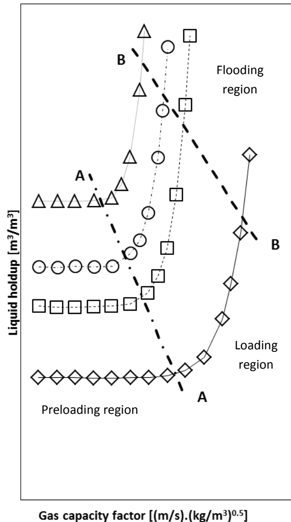
Fig. 3b. Liquid holdup evolution in a packing column.
