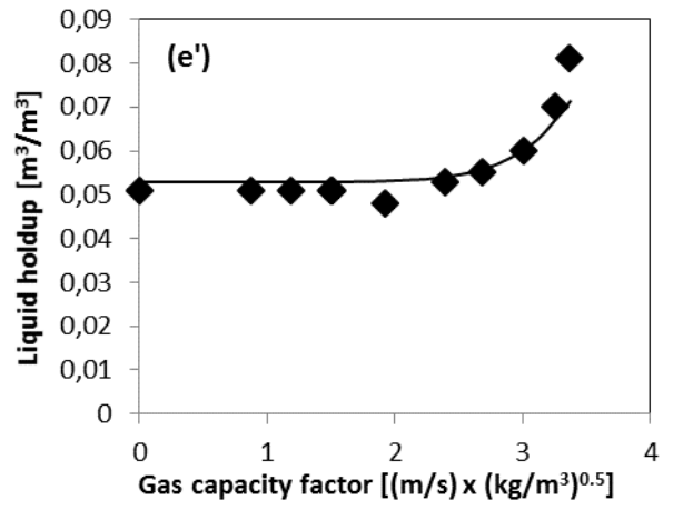
Fig. 6. Liquid holdup and pressure drop with an Air – Water system using Flexipac 350Y packing.
