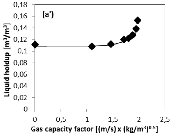
Liquid holdup
