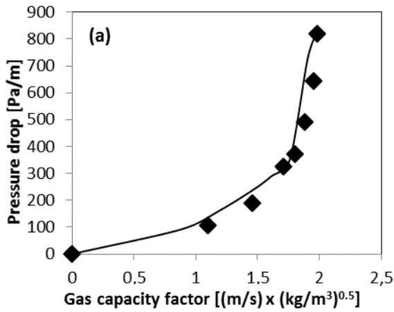
Pressure drop
