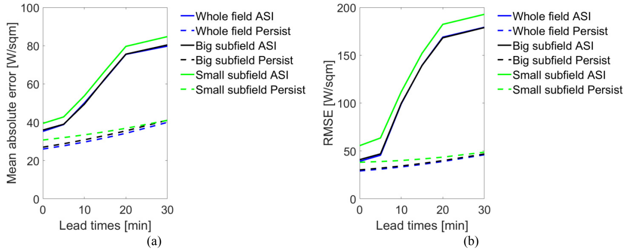
FIGURE 10. Statistical properties of the nowcasted DNI maps for different field sizes in comparison to the shadow camera reference system on Sept. 18 th 2015 . (a) Mean absolute error for the nowcasts (“ASI”, solid) and the persistence forecast (“Persist”, dashed) at different lead times and different field sizes. (b) RMSE error at different lead times and different field sizes.
