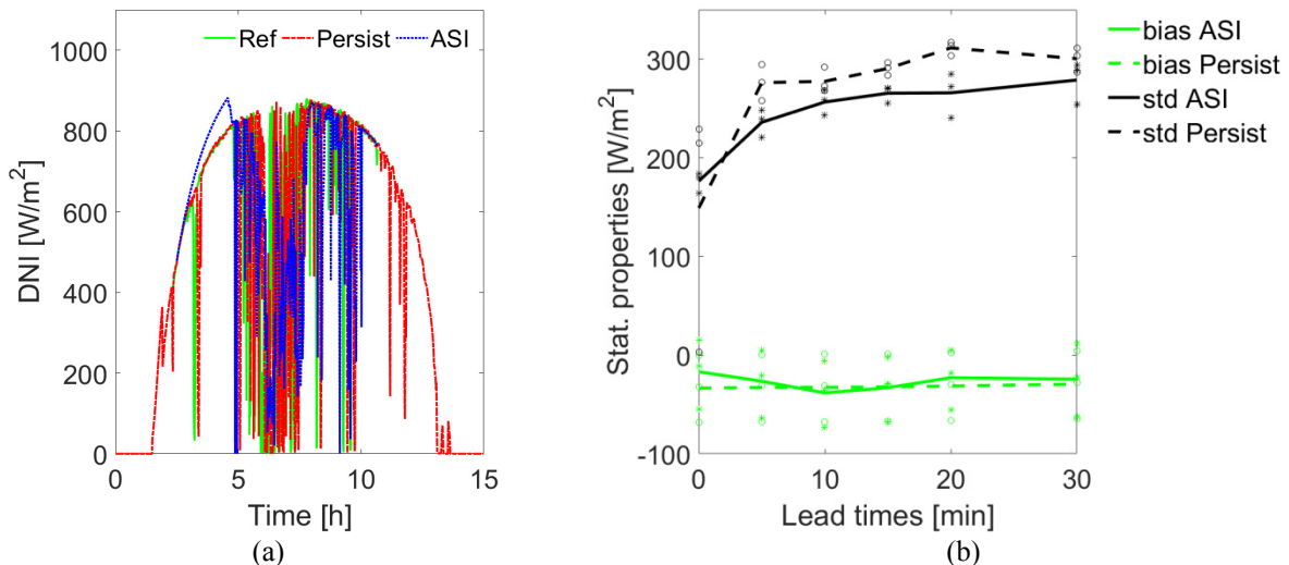
FIGURE 4. (a) DNI values of a reference station (green, solid), the persistence forecast (red, dashed) and the ASI-derived nowcasted values at the station’s position (blue, dotted) on Sept. 19 th 2015 . Persistence forecast and nowcasts have a lead time of 10 min. (b) Bias and standard deviation for the nowcasts (“ASI”, solid, stars) and the persistence forecast (“Persist”, dashed, circles) at different lead times. The values of three pyrheliometers are depicted as stars for the nowcasts and with circles for the persistence forecasts. The lines show the average of the results for the three pyrheliometers.
