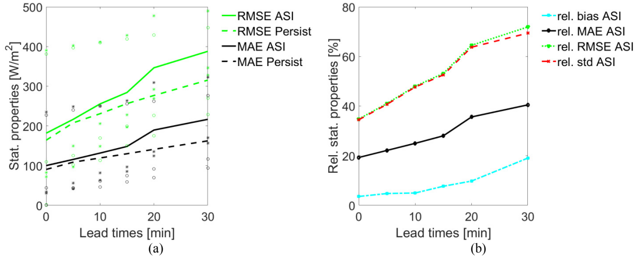
FIGURE 7. Statistical properties of the nowcasted DNI map-pixels in comparison to three pyrhemeters on Nov. 22 nd 2015. (a) RMSE and MAE for the nowcasts (“ASI”, solid, stars) and the persistence forecast (“Persist”, dashed, circles) at different lead times. The values of three pyrhemeters are depicted as stars for the nowcasts and with circles for the persistence forecasts. The lines show the average of the results for the three pyrhemeters. (b) Relative bias, relative MAE, relative RMSE and relative standard deviation of the nowcasts at different lead times.
