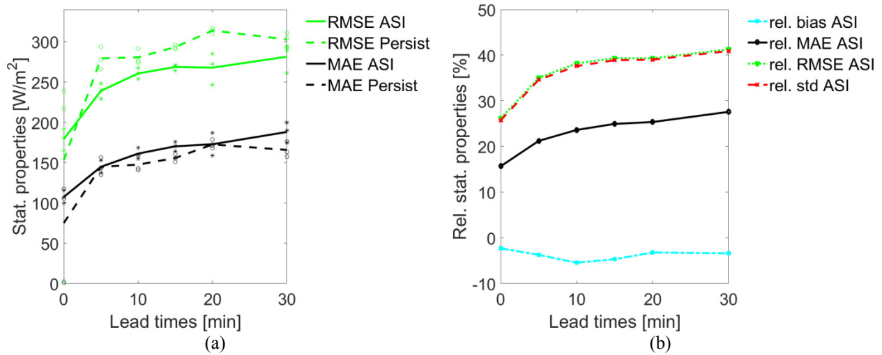
FIGURE 5. Statistical properties of the nowcasted DNI map-pixels in comparison to three pyr heliometers on Sept. 19 th 2015 . (a) RMSE and MAE for the nowcasts (“ASI”, solid, stars) and the persistence forecast (“Persist”, dashed, circles) at different lead times. The values of three pyr heliometers are depicted as stars for the nowcasts and with circles for the persistence forecasts. The lines show the average of the results for the three pyr heliometers. (b) Relative bias, relative MAE, relative RMSE and relative standard deviation of the nowcasts at different lead times.
