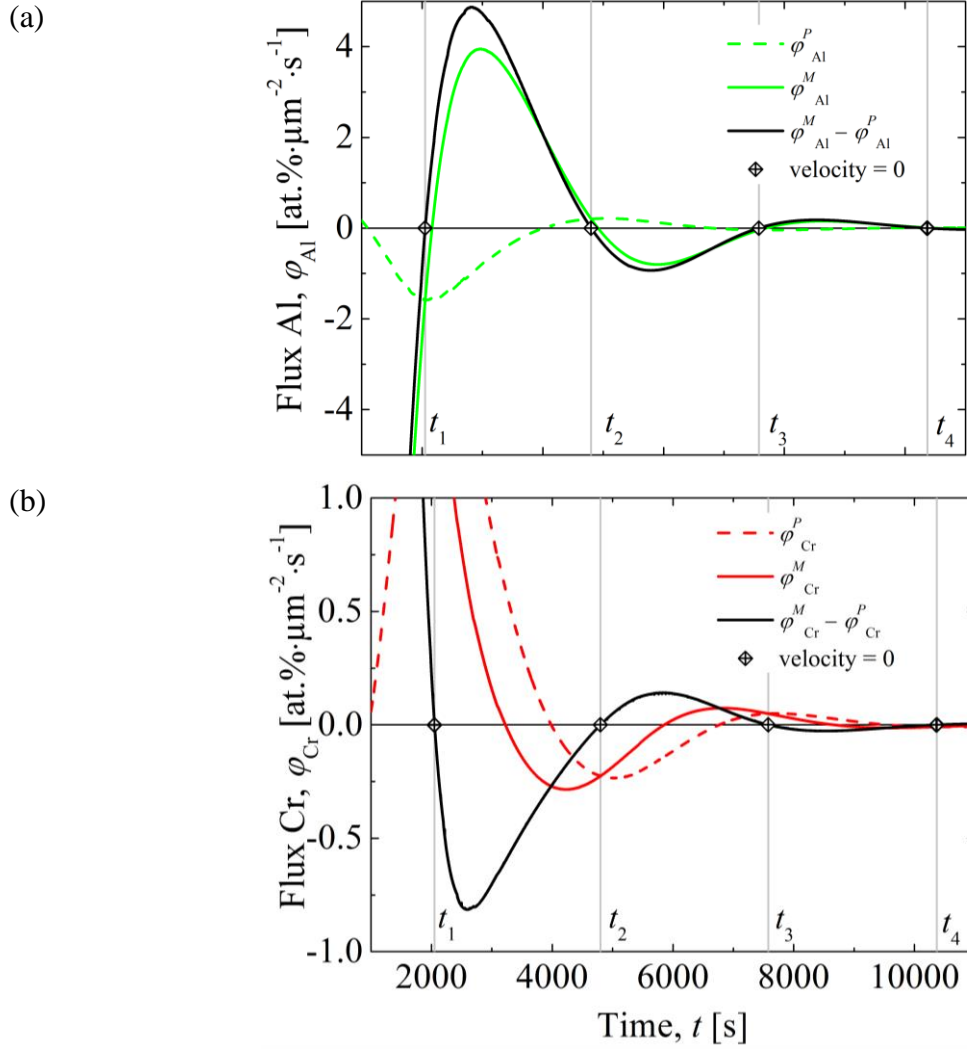
Figure 11: Time evolution of solute flux for (a) aluminum (Al) and (b) chromium (Cr) component at the M/P ( \gamma/\gamma' ) interface in front tracking computation developed with \mathbf{D}_{inf}^M diffusion matrix. The curvature effect on equilibrium compositions is considered. Diffusion fluxes are shown in both (plain lines) M - and (dashed lines) P - phase as defined by the Fick's law at the M/P interface. Differences between solute fluxes are presented in order to highlight the changes of the sign of the velocity. Symbols refer to the times t_i when velocity is equal to 0 also corresponding to a null value for the difference between solute fluxes. Values of solute fluxes in the two elements corresponding to these four times are reported in Table 6.
