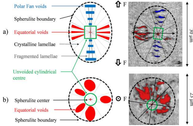
Figure 10. Diagrams of void arrangements within a deformed spherulite: (a) longitudinal view ( rz plane); (b) circumferential view ( r\theta plane).
