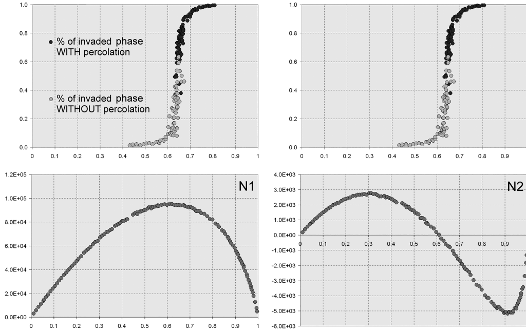
Fig. 3. Increasing numbers of 15 \times 15 squares uniformly placed on a hexagonal 2000 \times 2000 grid: the curves depicting the evolution of the topology and the percolation process are compared as a function of the compacity.
