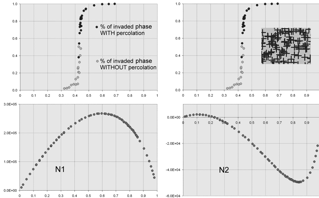
Fig. 8. Increasing numbers of crosses (width 21, thickness 3) are uniformly placed on a hexagonal 2000*2000 grid. The percolation threshold does not match with any of the singular points of the curves depicting the topological evolution of the structure.
