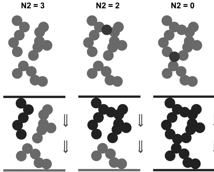
Fig. 1. (Top) An increase of the number of connections modifies the topology of the phase which, in turn, leads to a decrease of the values of the EPC ( N2 ). (Bottom) As the black phase is getting more and more connected, its invasion by a fluid (from the top to the bottom of the field) is more and more complete.
