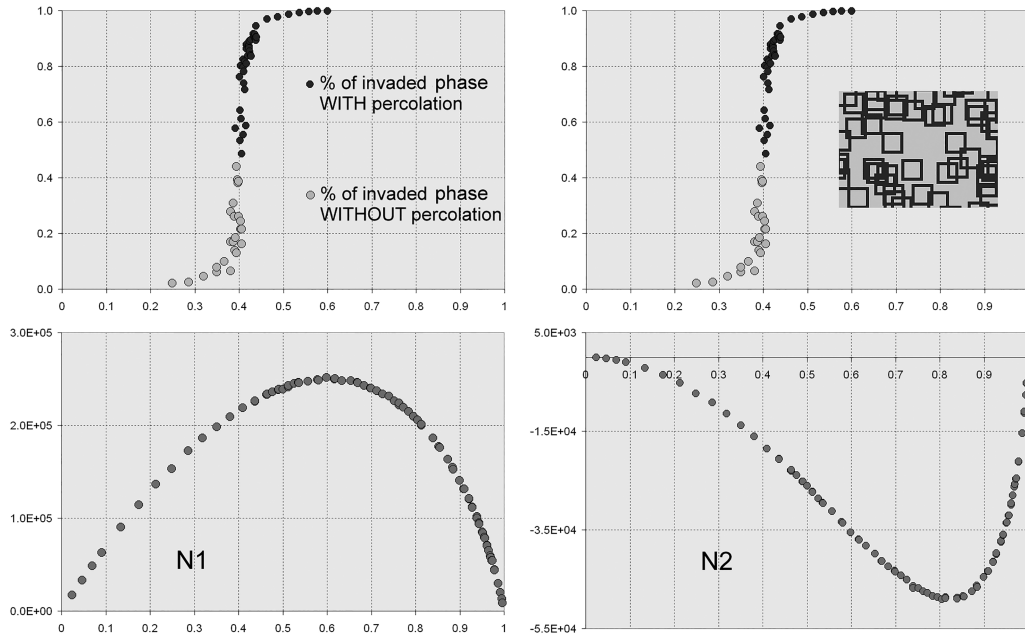
Fig. 7. Increasing numbers of square crowns (outer width 21, thickness 3) are uniformly placed on a hexagonal 2000*2000 grid. The percolation threshold does not match with any of the singular points of the curves depicting the topological evolution of the structure.
