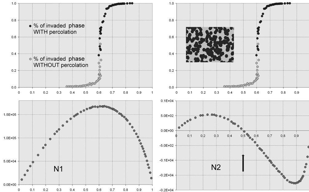
Fig. 5. Structures obtained by applying a dilation of size 5 on increasing numbers of points uniformly distributed on the grid. A coincidence is observed between the percolation threshold and the maximum of N1 but no longer with the zero value of N2 (arrow).
