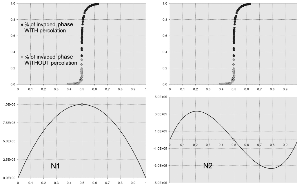
Fig. 4. Increasing numbers of points uniformly distributed on a hexagonal 2000 \times 2000 grid: a coincidence is observed between the maximum of N1, the zero and the inflection point of N2 and the percolation threshold.
