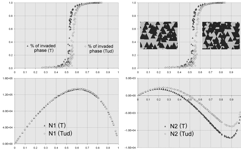
Fig. 9. Two procedures are used to fill progressively the space with triangles (edge 20): uniform implantation of up pointing triangles (T) and mixture of half-half up and down pointing triangles (Tud). For these two simulations, two different percolation transitions are observed (upper curves). As far as the topological properties are concerned (lower curves), the thresholds correspond neither to the zeros of N2 nor to the compacity of the maximum of N1 for which a single curve is obtained.
