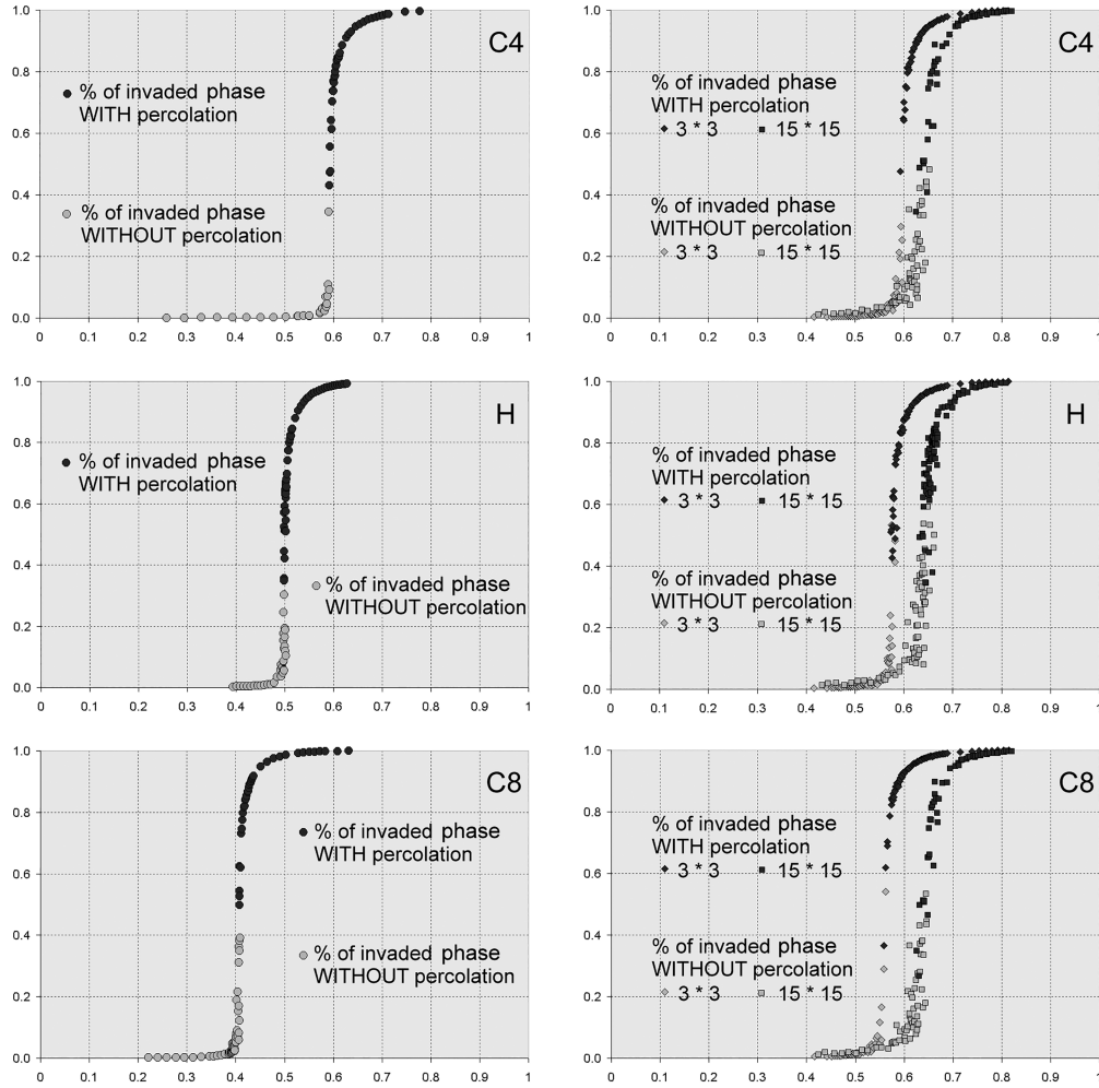
Fig. 2. (Left) Propagations through increasing numbers of points uniformly distributed on 2000*2000 grids using a 4-connectivity square grid (top), 6-connectivity hexagonal grid (middle) or 8-connectivity square grid (bottom) lead to three different percolation thresholds. (Right) Propagations through increasing numbers of monosized squares (3*3 or 15*15) uniformly distributed on 2000*2000 grids using a 4-connectivity square grid (top), 6-connectivity hexagonal grid (middle) or 8-connectivity square grid (bottom) lead to the same percolation threshold only for the 15*15 squares. For all curves, the percentage of invaded area is plotted as a function of the compacity
