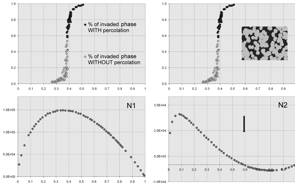
Fig. 6. Structures obtained by applying a closure of size 5 on increasing numbers of points uniformly distributed on the grid. A coincidence is observed between the percolation threshold and the maximum of N1 but no longer with the zero value of N2 (arrow).
