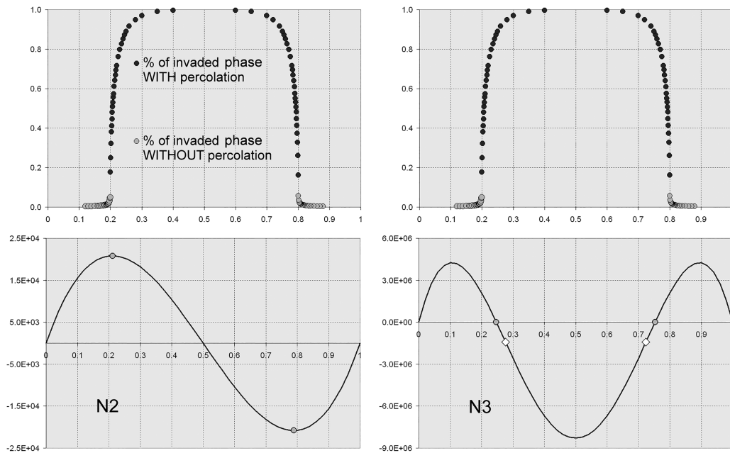
Fig. 10. Increasing numbers of points uniformly distributed on a face-centered-cubic 500*500*500 grid (the natural 12-connectivity of the f.c.c. grid has been used for the propagations and the theoretical curves of the EPC represented here could have been obtained by sweeping the whole space with the rhomboedral unit of the f.c.c. grid). The compacities for which the two percolation thresholds occur are about 0.2 and 0.8 in the vicinity of the extrema of N2.
