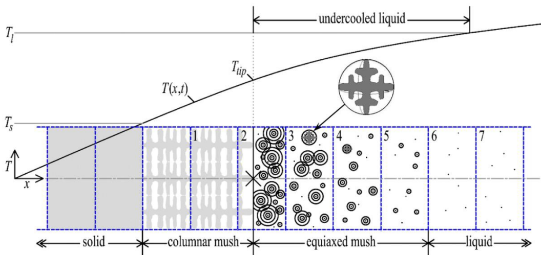
Fig. 5: Spherical equiaxed envelopes growing in undercooled liquid and positive temperature gradient ahead of a columnar front (×) in the BFFTM domain
