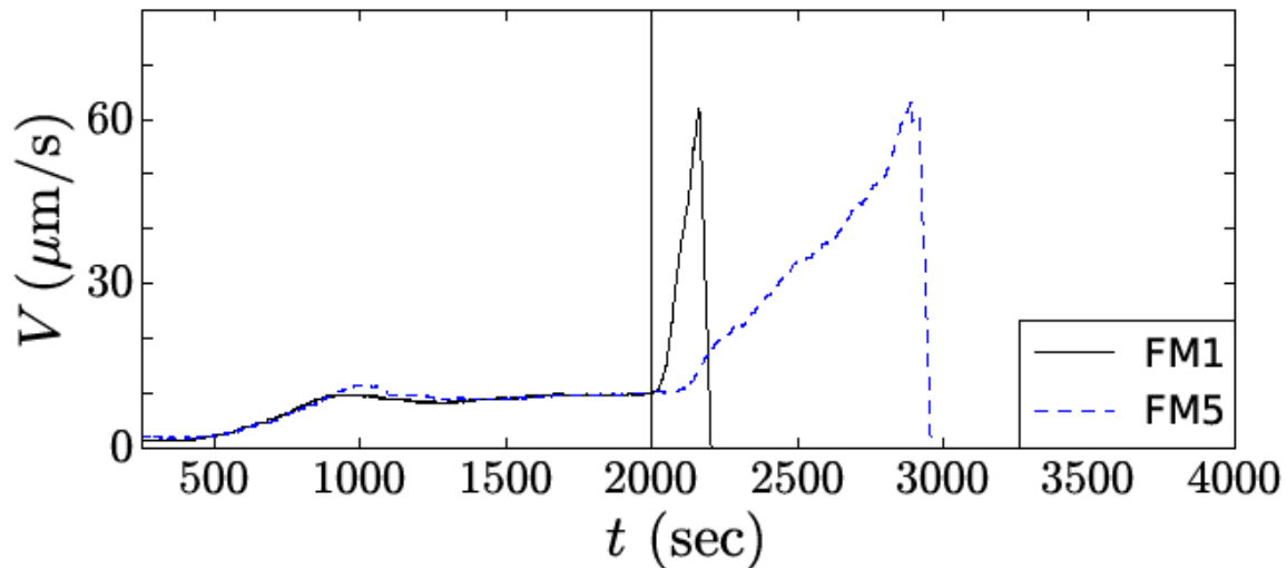
Figure 8: Time evolution of the velocity of the most advanced columnar front for Batch1 FM1 and FM5 in DNN simulations. The front velocity increases during the growth competition of columnar dendrites leading to an increase of primary spacing ( t < 1000 s). After this transient regime, the columnar front grows at a constant velocity. The front velocity increases again upon faster cooling during stage II and drops abruptly when columnar growth is blocked by the nucleated equiaxed grains.
