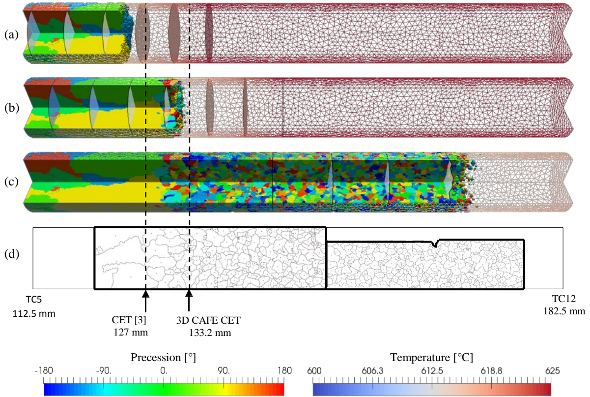
Figure 6: CAFE simulation of the solidification grain structure of the B1-FM1 sample between thermocouples TC5 (112.5 mm) and TC12 (182.5 mm). Isothermal surfaces from 602 °C to 626 °C with a step of 4 °C are shown. A quarter of the cylinder was removed by post-processing in order to offer an exploded view at various times of (a) columnar growth at t = 1,800 s, (b) nucleation and growth of equiaxed grains triggered by a sudden increase of the withdrawal rate at t = 2,140 s and (c) the equiaxed structure forming at t = 2,400 s. The position of the CET favourably compare with the (d) experimental grain structure observed in a longitudinal metallographic cross section [3].
