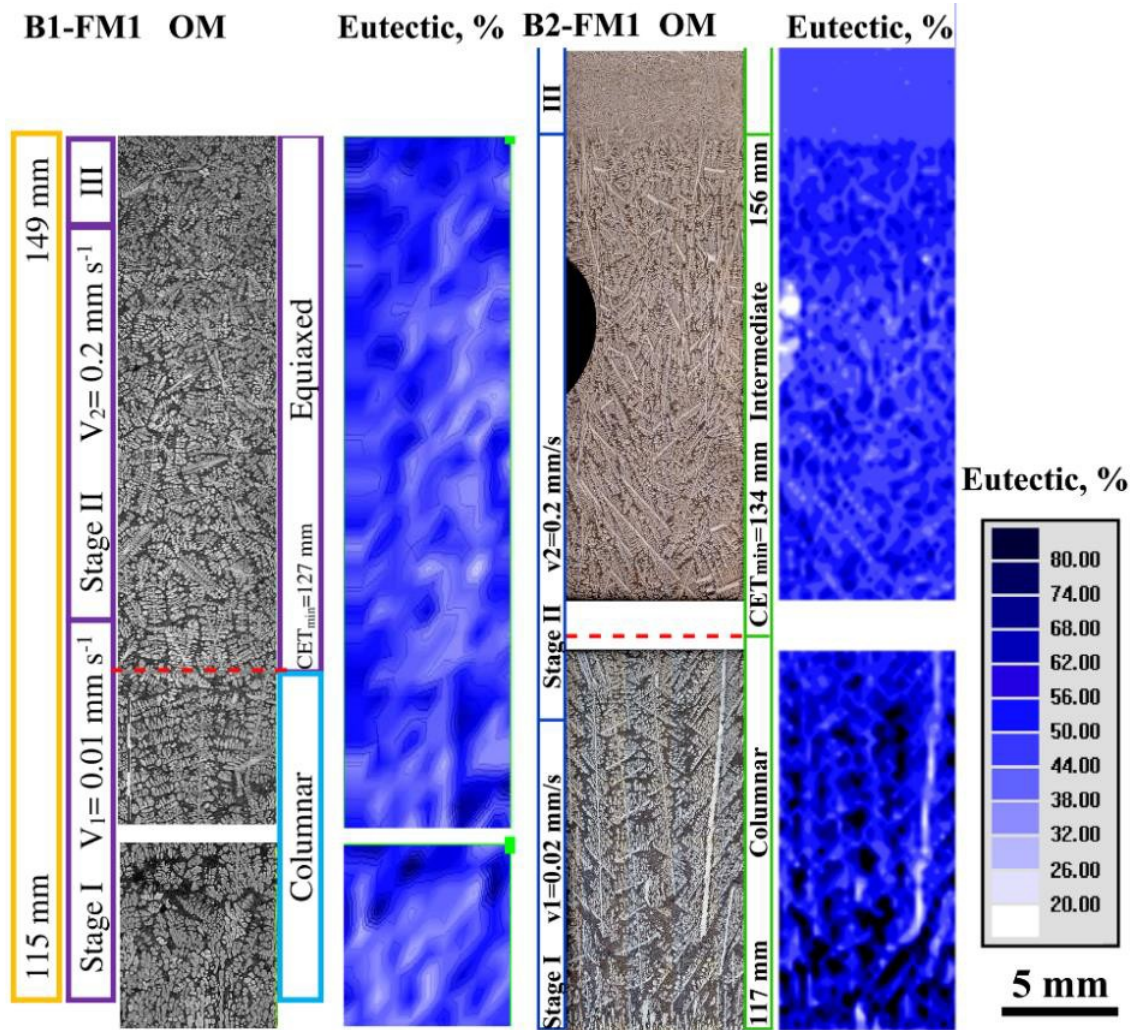
Fig. 2: Longitudinal microstructures by optical microscopy OM (left) and eutectic percentage distribution maps (right) for flight samples B1-FM1 and B2-FM1. The blank region represents the material loss during sample preparation.
