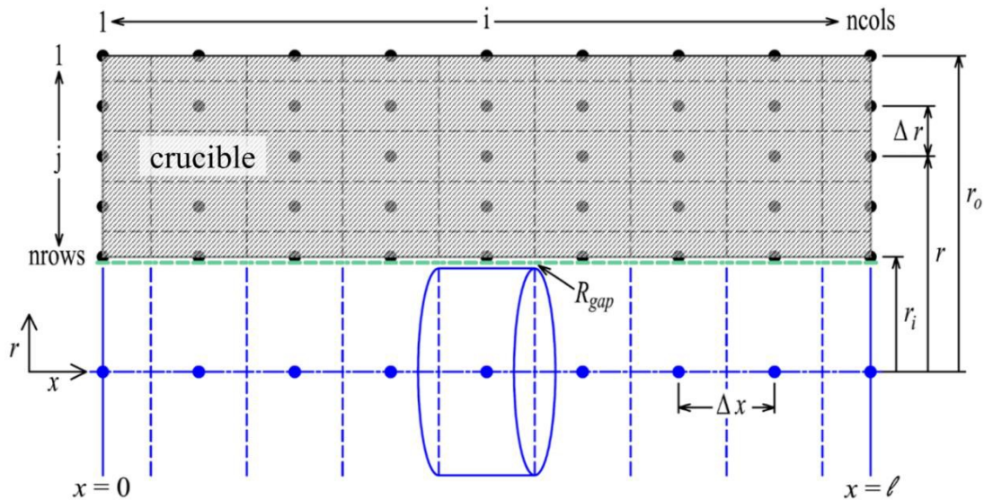
Fig. 4: BFFTM domain with 2-dimensional axisymmetric crucible.
