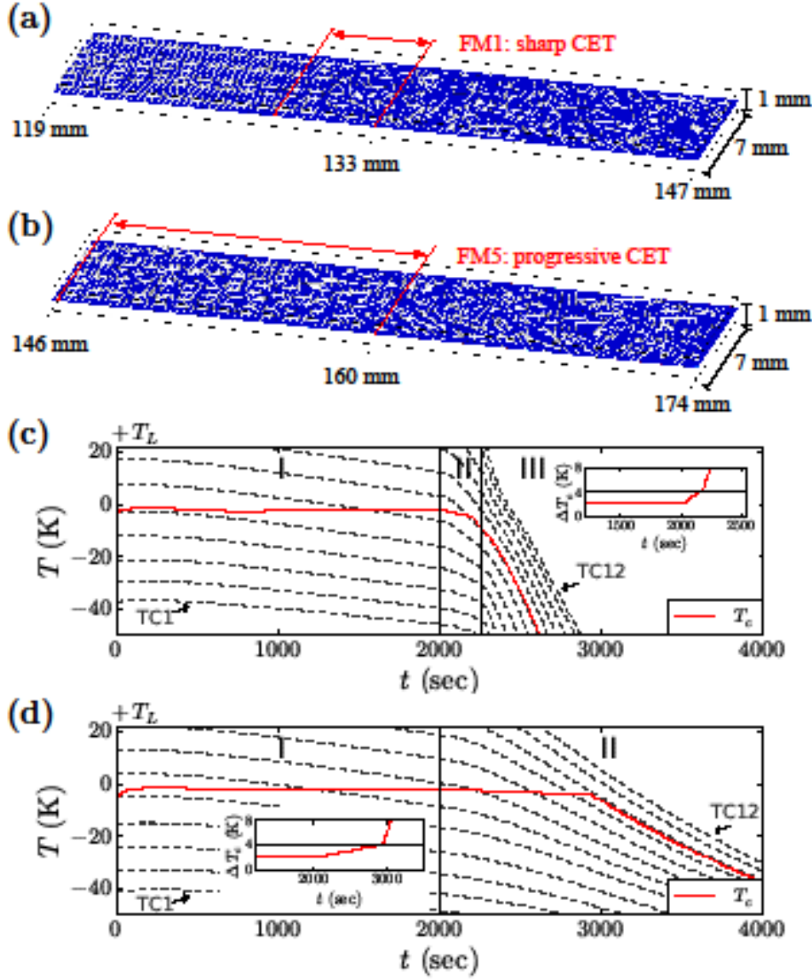
Fig. 7: DNN simulations of dendritic network and grain structures for Al-7wt%Si samples for B1-FM1 (a) and B1-FM5 (b) samples (see Table 1). A sharp CET is observed in FM1 ( CET_{min} = 125\text{mm} and CET_{max} = 129\text{mm} ) and a more progressive CET is observed in FM5 ( CET_{min} = 130\text{mm} and CET_{max} = 156\text{mm} ) [2]. (c) and (d) show the temperature curves recorded from 12 thermocouples (thin black dashed lines labelled TC1 to TC12) and the temperature of the most advanced columnar front T_c (solid red lines) in FM1 (c) and FM5 (d). The insets of (c) and (d) show zoomed in views of the time evolution of the columnar front undercooling \Delta T_c . The solid line represents the nucleation undercooling \Delta T_n = 4 K, which is used in simulations.
