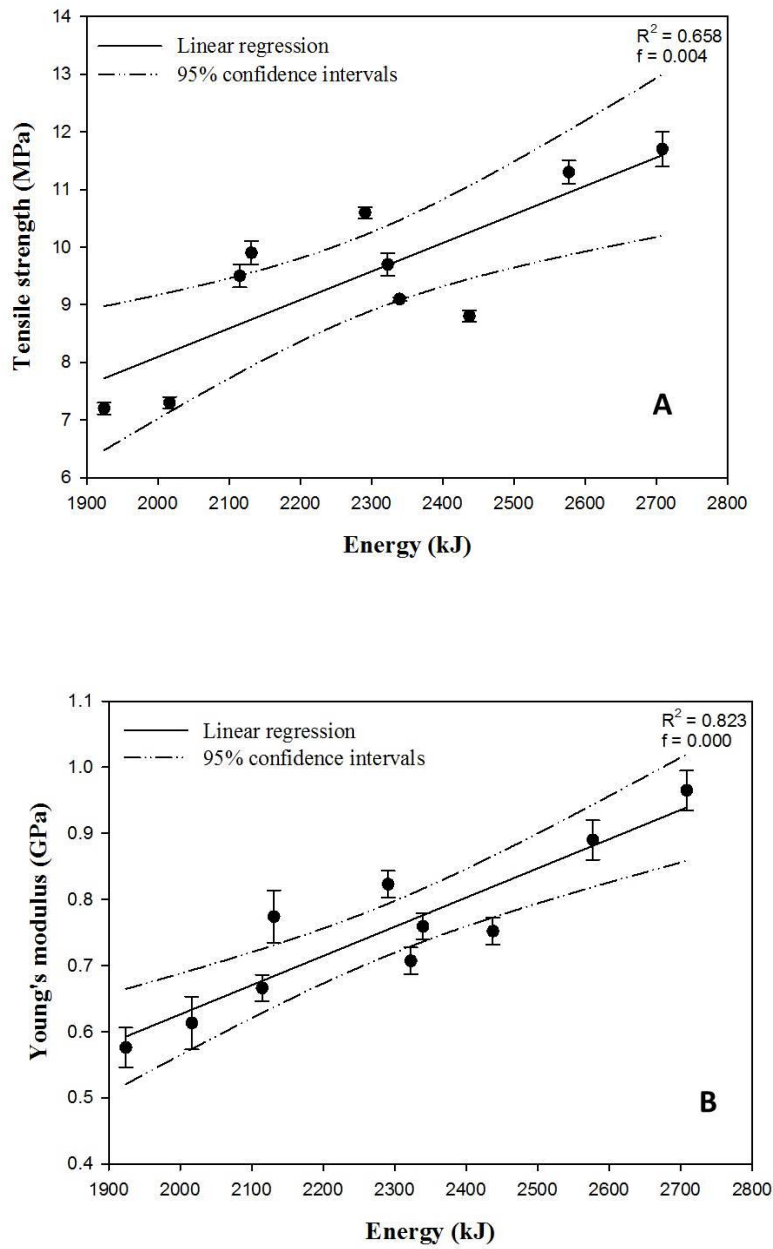
Figure 8. Correlations between energy consumed during compounding and tensile strength of composites (A) and energy consumed during compounding and Young's modulus (B) of the composites, for the ten genotypes.
