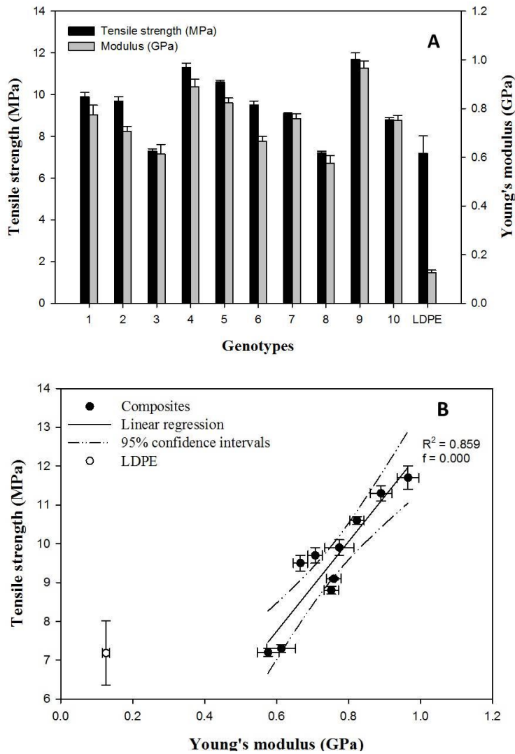
Figure 6. Tensile strength and Young's modulus of the LDPE-sorghum reinforced composites (standard errors correspond to five test bar replicates per genotype) (A) and the relationship between the two parameters (B).
