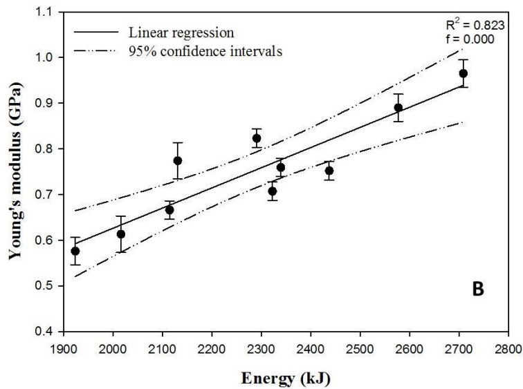
Figure 8. Correlations between energy consumed during compounding and tensile strength of composites (A) and energy consumed during compounding and Young's modulus (B) of the composites, for the ten genotypes.
