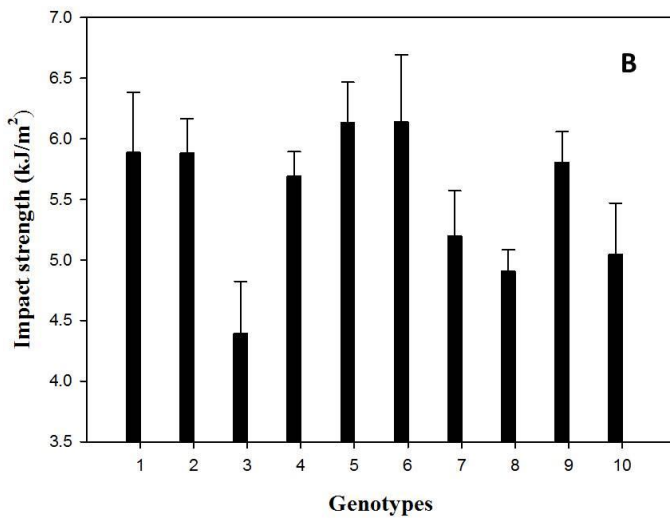
Figure 7. Elongation at break (elongation at break of LDPE was not detected) (A) and notched impact strength of sorghum-LDPE reinforced composites (notched impact strength of LDPE = 44.7 \pm 1.1 (kJ/m 2 )) (B). Standard errors correspond to five test bar replicates per genotype.
