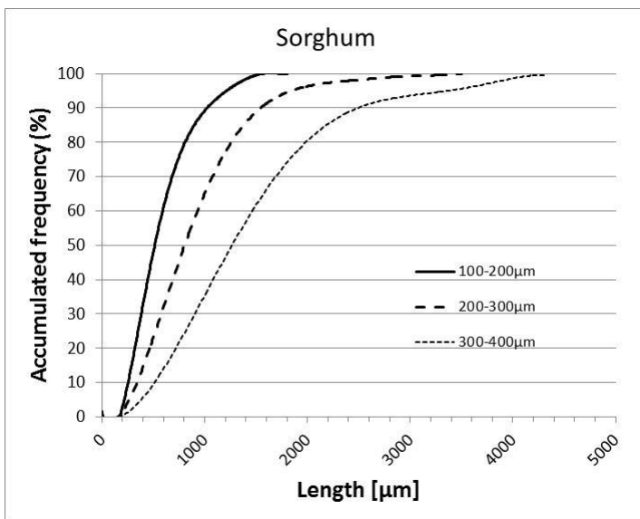
Figure 2. Size distribution of sorghum stem fragments collected at three different sieves (between 100 and 200 \mu\text{m} , 200 and 300 \mu\text{m} and 300 and 400 \mu\text{m} ) in terms of length (left hand side graph) and aspect ratio (right hand side graph) for one sorghum genotype (BIOMASS140, genotype 7).
