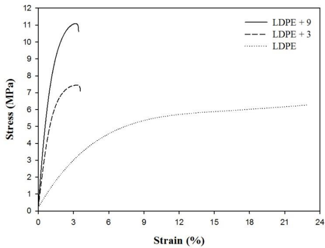
Figure 5. Stress/strain curves of the LDPE and two composites produced with genotypes 3 (IS26731) and 9 (RE1).
