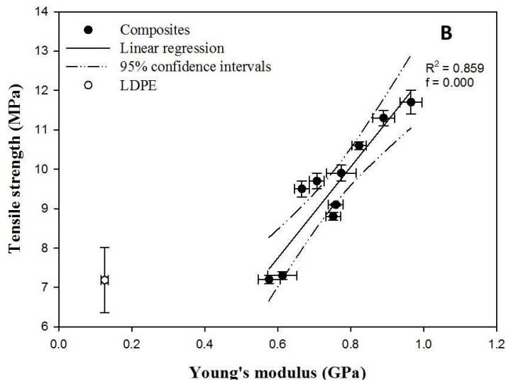
Figure 6. Tensile strength and Young's modulus of the LDPE-sorghum reinforced composites (standard errors correspond to five test bar replicates per genotype) (A) and the relationship between the two parameters (B).
