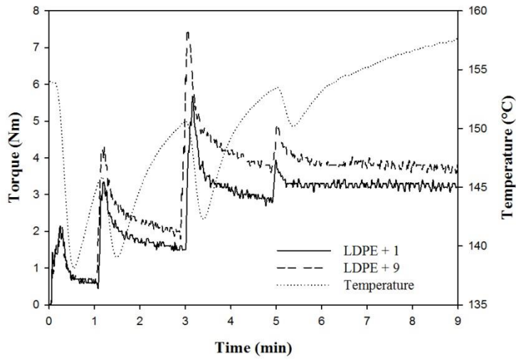
Figure 4. Torque-temperature-time curves during compounding of sorghum stems with LDPE. LDPE+1 and LDPE + 9 are two different compounding experiments with genotypes 1 (IS19453) and 9 (RE1).
