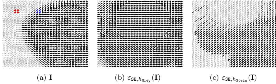
Fig. 2. Background and foreground sets are blue and red ellipses in (a). Note that the erosion by h_{\text{Grey}} causes a colour homogenisation in comparison to an orientation uniformity by h_{\text{Stein}} . SE is a disk of diameter 20 pixels.
