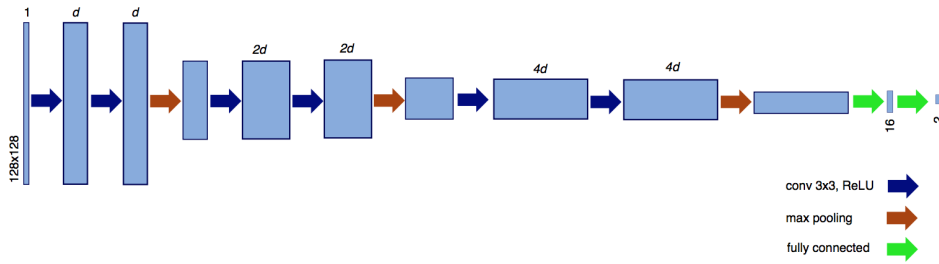
Figure 1: Schematic representation of the CNN that we used in the work here presented. It comprises 6 convolutional layers. Three max-pooling layers and 2 fully connected layers.
