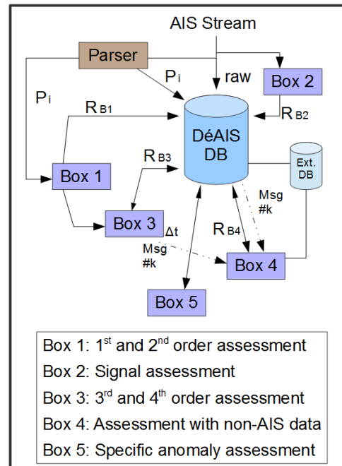
Figure 3: Proposed architecture
