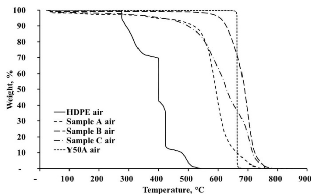
Fig. 4. TGA curves obtained for the three plasma carbon back samples, the HDPE pellets and the industrial carbon black sample (Y50A). TGA conditions: 900^\circ\text{C} in air @ 30^\circ\text{C}\cdot\text{min}^{-1} HR5, S1
