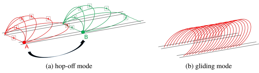
Figure 7: Schematic decomposition of observed arc dynamics: for the hope-off mode 0 \Rightarrow 1 \Rightarrow 2 "stretching", 2 \Rightarrow 3 \Rightarrow 4 \Rightarrow 5 "tilting", 0 \Rightarrow "restriking"
