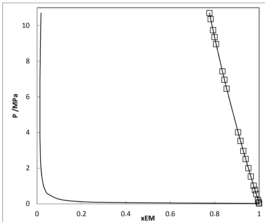
Figure 3 Phase diagram ( P - x - y ) of methane-EM binary system at 272K, symbol: experimental data [12], Lines: adjusted data obtained with PR-CPA EoS.
