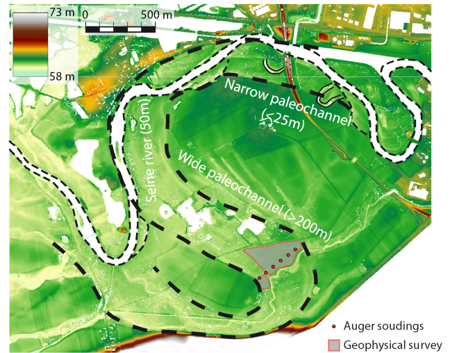
Figure 2. Lidar map of the study area, showing the contemporary location of the Seine River, together with the narrow and wide paleochannel interpretations.
