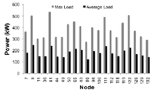
Figure 4: Maximum and average load for indicated nodes
