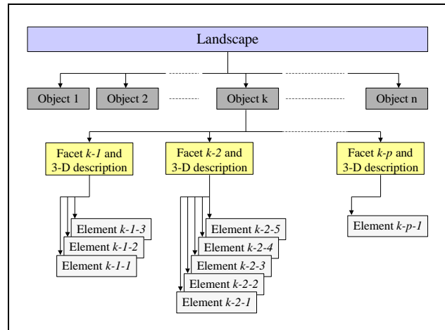
Figure 2: illustration of the landscape element representation.
