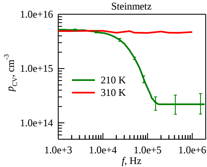
Fig. 8 Apparent concentration vs. frequency for Steinmetz sample; T = 210 and 310 K. Error bars are shown
