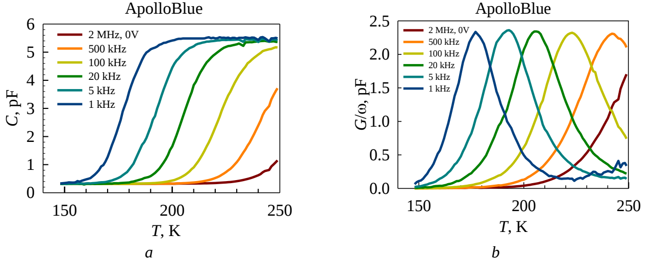
Fig.5 C - T (a) and G/\omega - T (b) spectra, Apollo Blue
