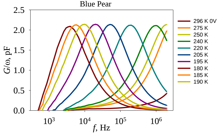
Fig.6 G/\omega - f spectra for Blue Pear
