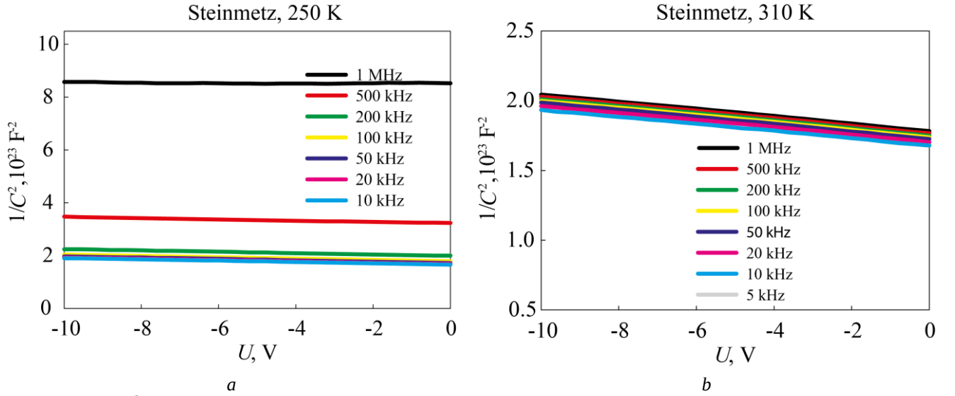
Fig. 4 1/C^2 -V characteristics for the Steinmetz blue diamond sample at: a) 250 K – non-quasistatic condition; b) 310 K – quasistatic condition
