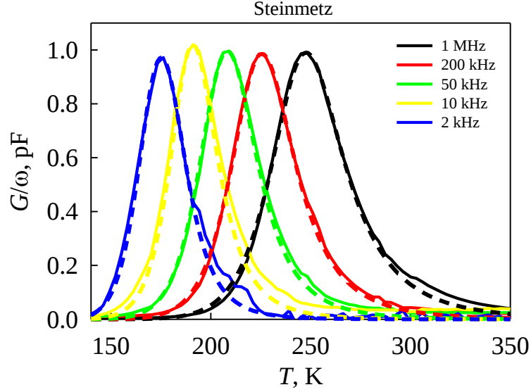
Fig.7 Experimental (solid line) and modeled (dashed line) G/\omega vs. T spectra for Steinmetz sample at various frequencies
