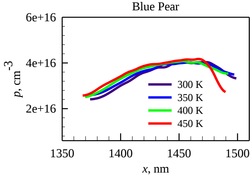
Fig.9 Carrier concentration profiles at different temperatures, Blue Pear diamond
