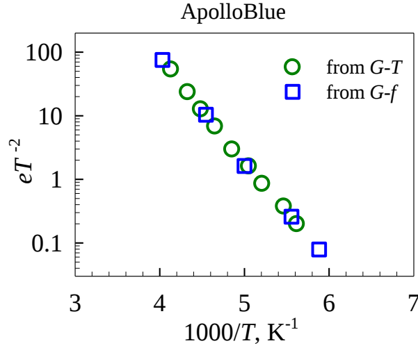
Fig. 10 Arrhenius plot for Apollo Blue from G-T and G-f spectra
