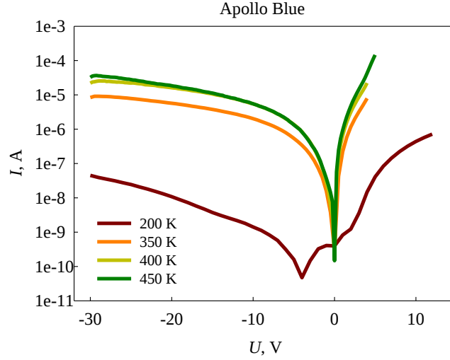
Fig.3 Typical I - V characteristics for the natural Apollo Blue diamond sample at various temperatures (abs value for I is used)
