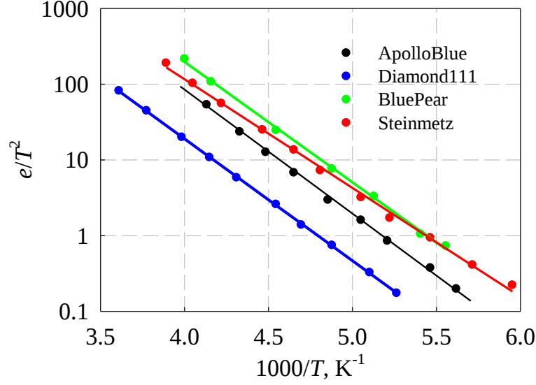
Fig.11 Arrhenius plots for all samples
