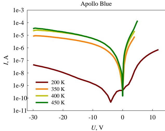
Fig.3 Typical I - V characteristics for the natural Apollo Blue diamond sample at various temperatures (abs value for I is used)
