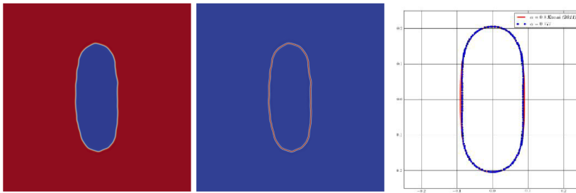
Figure 10: Level set function, Dirac function and the reference solution for \eta = 0.77
