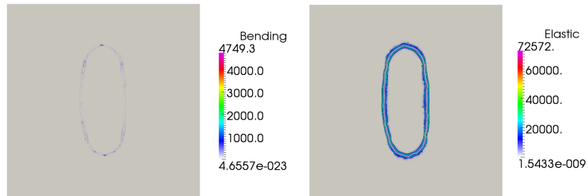
Figure 13: The bending and the elastic forces for \eta = 0.77
