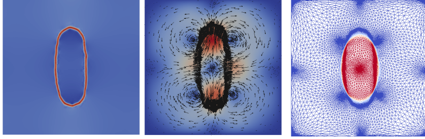
Figure 16: The pressure, velocity and the adapted mesh obtained for \eta = 0.77
