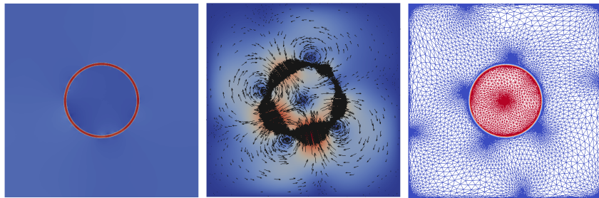
Figure 14: The pressure, velocity and the adapted mesh obtained for \eta = 1
