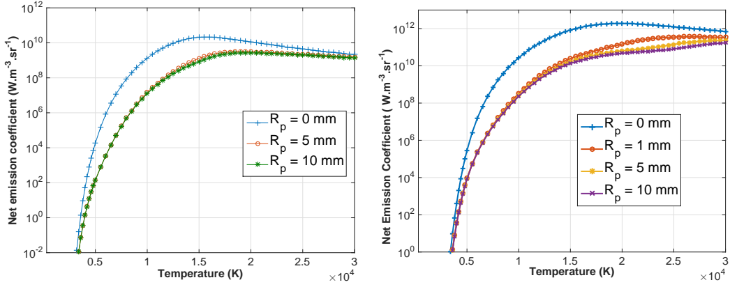
Figure 4: NEC of hydrogen plasma at 1 bar and for different plasma thicknesses
