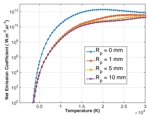
Figure 5: NEC of hydrogen plasma at 20 bar and for different plasma thicknesses
