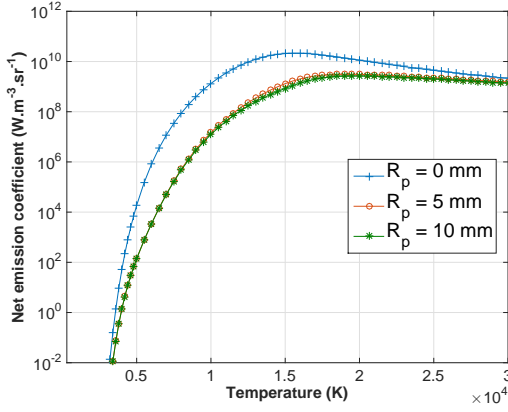
Figure 4: NEC of hydrogen plasma at 1 bar and for different plasma thicknesses
