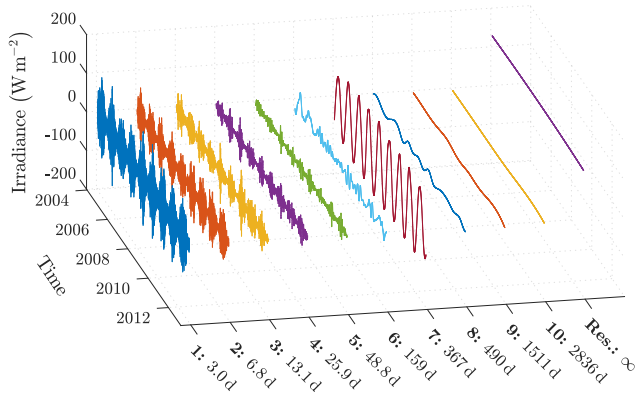
Figure 2. The IMFs obtained by decomposing the WRDC time-series for VIE, plotted as YZ slices, with the x axis denoting their number (IMF1... IMF10) and mean time-scales in days. For reference, the residual (Res.) is also included. The amplitude, or irradiance, of each IMF is plotted on the z axis, and time runs on the y axis. Time markers denote 1 January of the corresponding year.
