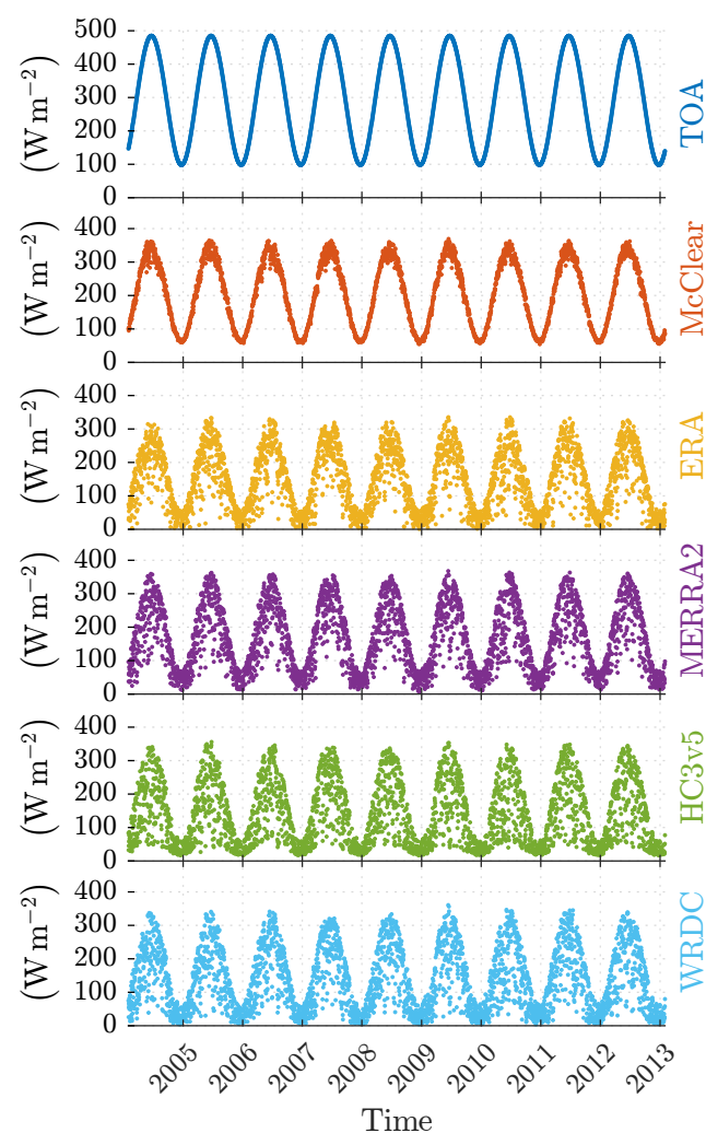
Figure 1. The six solar irradiance time-series for VIE investigated in this study, spanning 1 February 2004 to 31 January 2013. From top to bottom: TOA, McClear, ERA, MERRA2, HC3v5, and WRDC. Each point corresponds to a daily mean of irradiance. Time markers on the abscissa indicate the start of the corresponding year.
