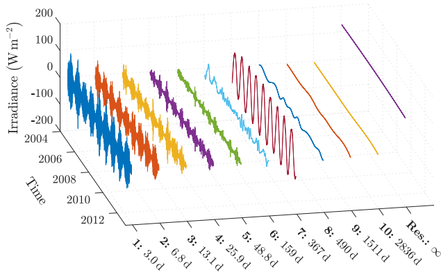
Figure 2. The IMFs obtained by decomposing the WRDC time-series for VIE, plotted as YZ slices, with the x axis denoting their number (IMF1...IMF10) and mean time-scales in days. For reference, the residual (Res.) is also included. The amplitude, or irradiance, of each IMF is plotted on the z axis, and time runs on the y axis. Time markers denote 1 January of the corresponding year.
